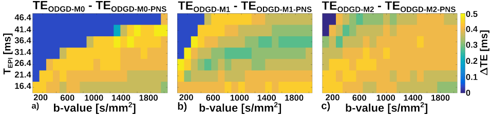
Figure 5.3: TE reductions ( \Delta TE ) achieved using ODGD- M_n -PNS compared to ODGD- M_n for b -values 100 - 2000s/mm 2 and T_{EPI} in the range of 16.4 - 46.4 ms for M_0 (a), M_1 (b) and M_2 (c) moment constraints, respectively. There is a TE reduction between 0 - 0.94%, 0 - 0.74% and 0 - 0.75% for M_0 , M_1 and M_2 , respectively. TE reductions are comparable throughout b -value, T_{EPI} ranges, and n th-order moment-nulling. ODGD- M_n and ODGD- M_n -PNS were computed with SRMax of 100 T/m/s (limit found on the literature to avoid PNS-effects) and 150 T/m/s (hardware limit), respectively.
